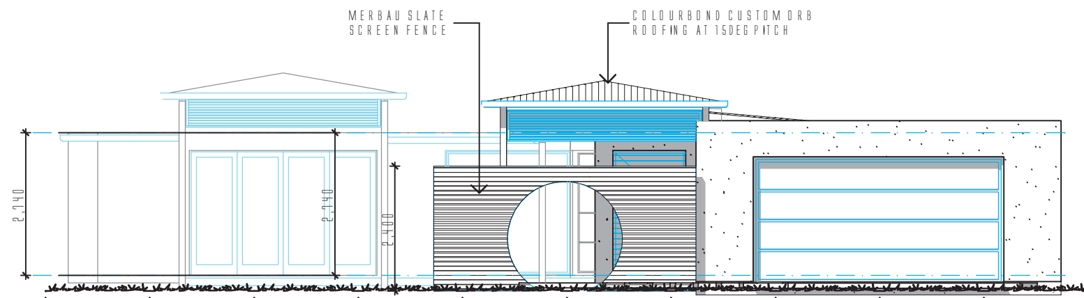
WEST ELEVATION
