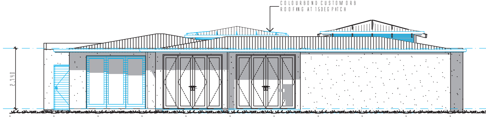
EAST ELEVATION
