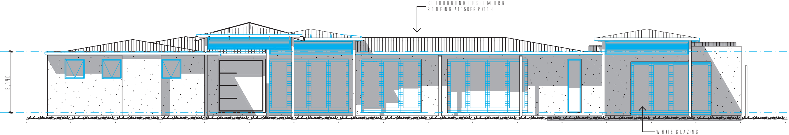
NORTH ELEVATION
